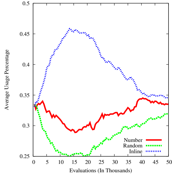
Figure 1.6: Primitive parameter usage on DTrap
