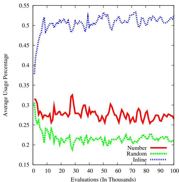
Figure 1.5: Primitive parameter usage on Offset Rastrigin
